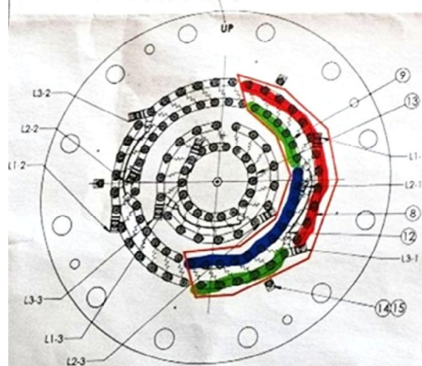
WIRING DIAGRAM 3 PH DELTA, 3 CIRCUITS SCALE 1:4
