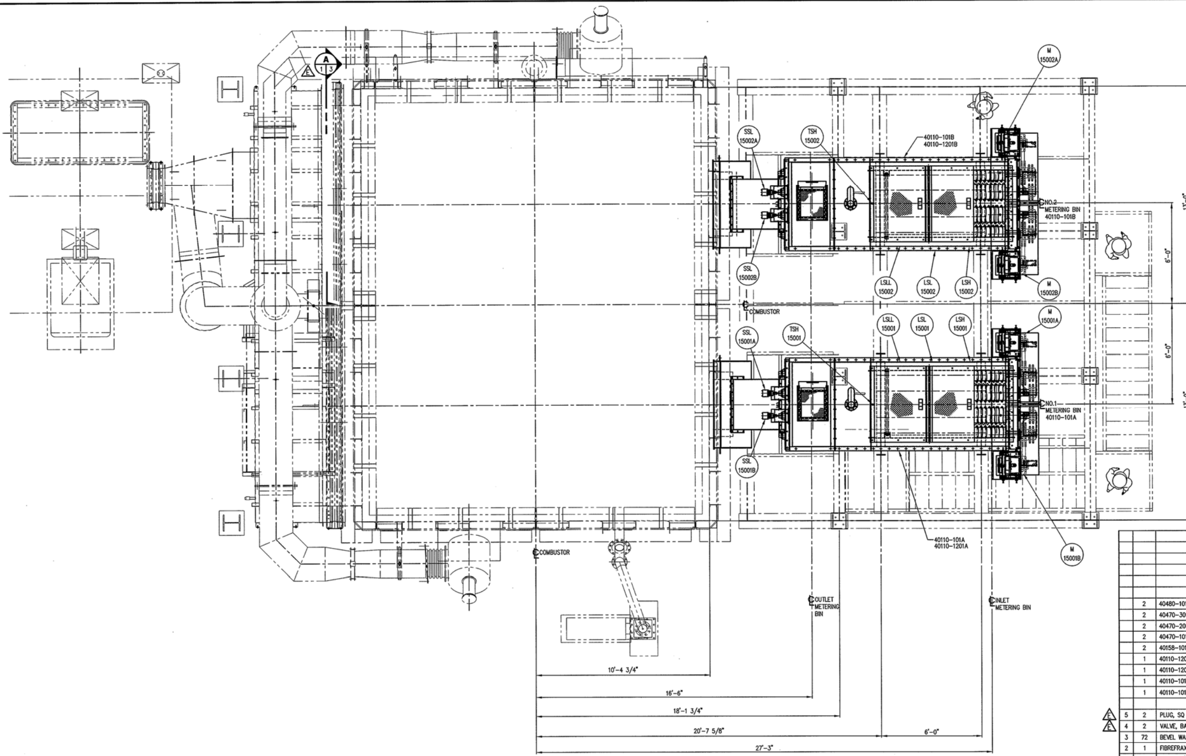
PLAN VIEW 3/8" = 1'-0"
