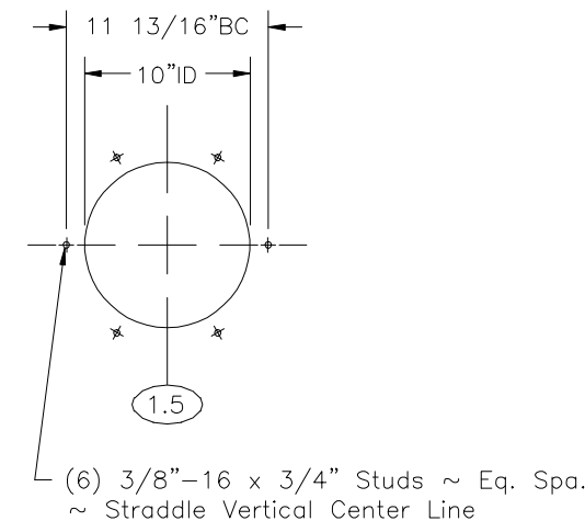
Negative Air Flange Detail
